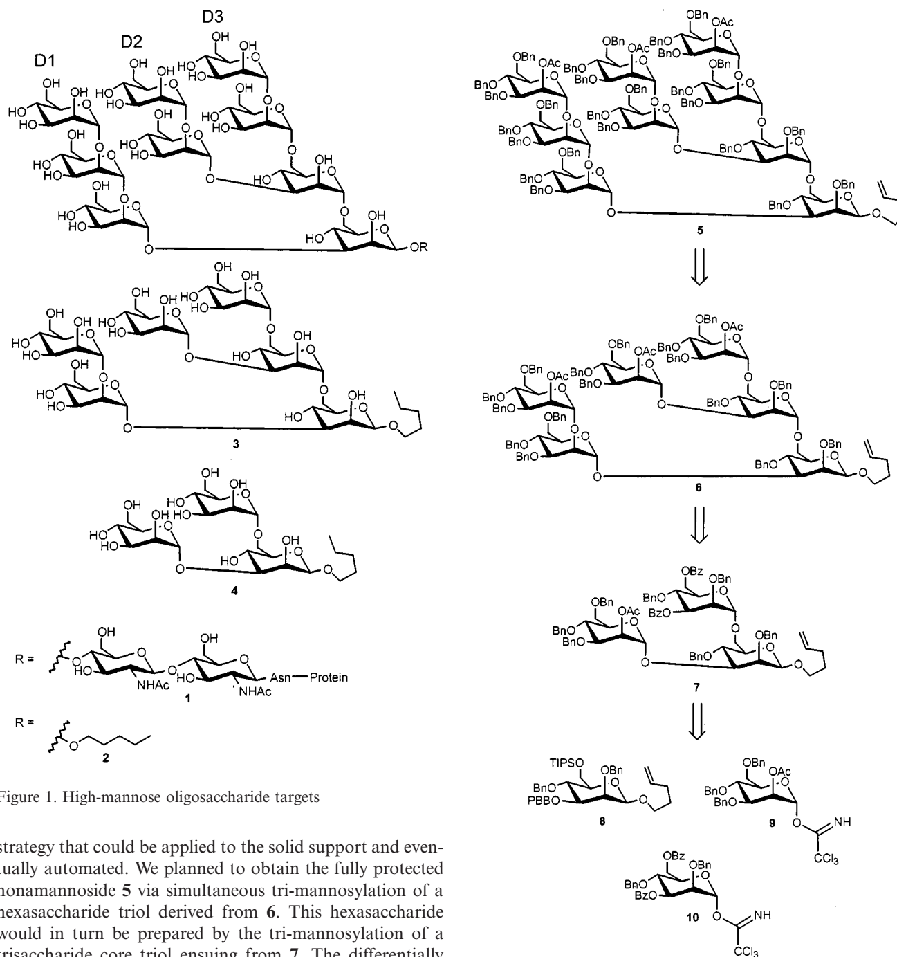
Scheme 1. Retrosynthesis of nonamannoside 5
