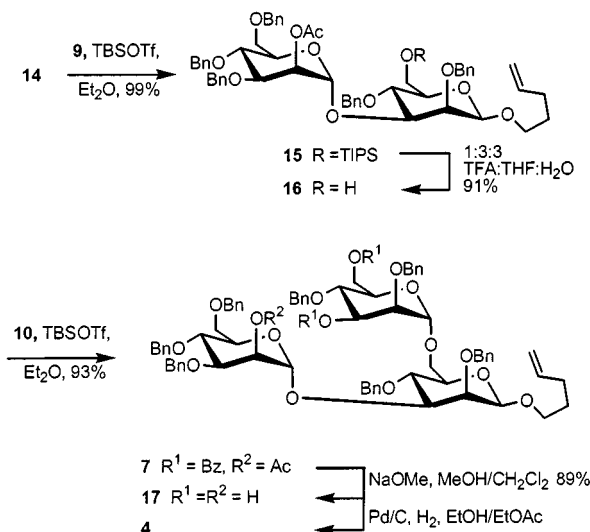
Scheme 3. Assembly of core trimannoside 7
