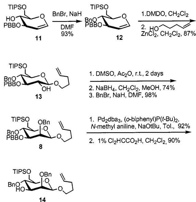
Scheme 2. Synthesis of the core \beta -mannoside 8
